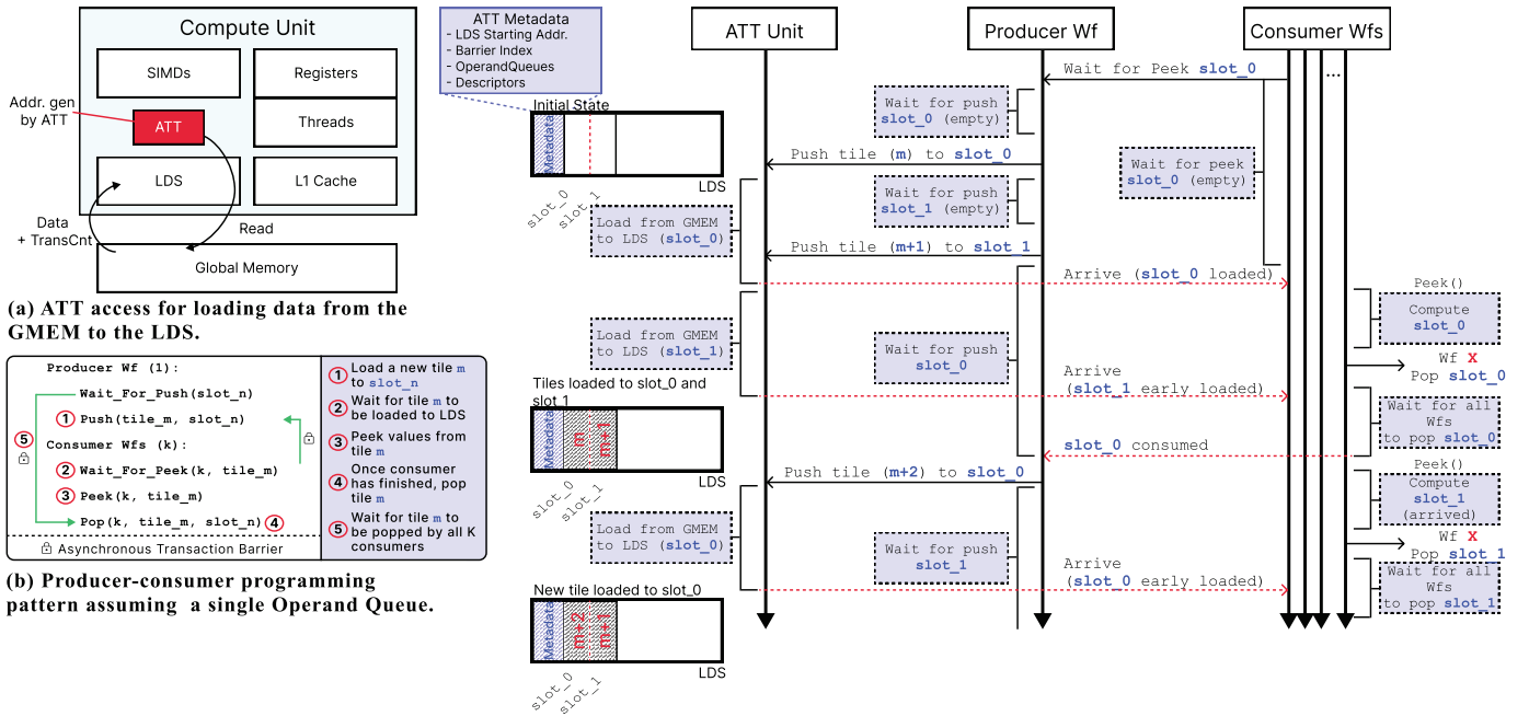
Fig. 2: Use of the ATT unit with the Operand Queue library that constitutes the baseline in this work.
