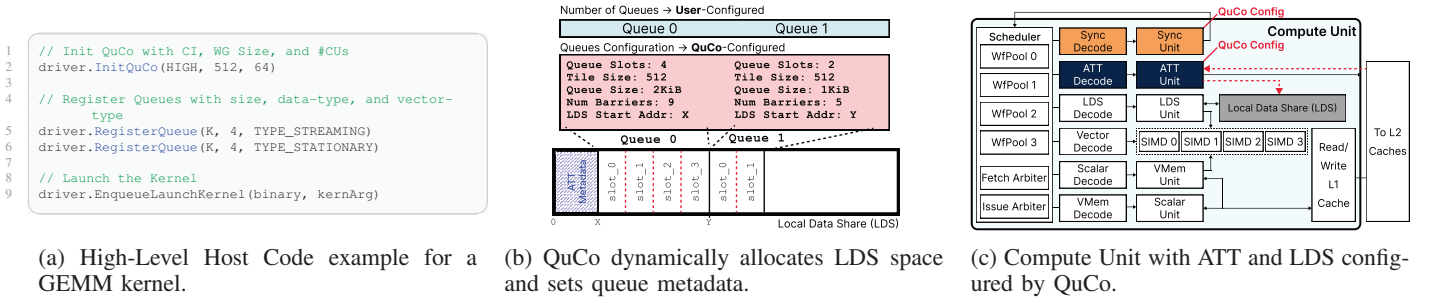
Fig. 4: Example of QuCo for two operand queues (Queue 0 and 1) at: (a) software-level (b) queue level; (c) hardware level.
