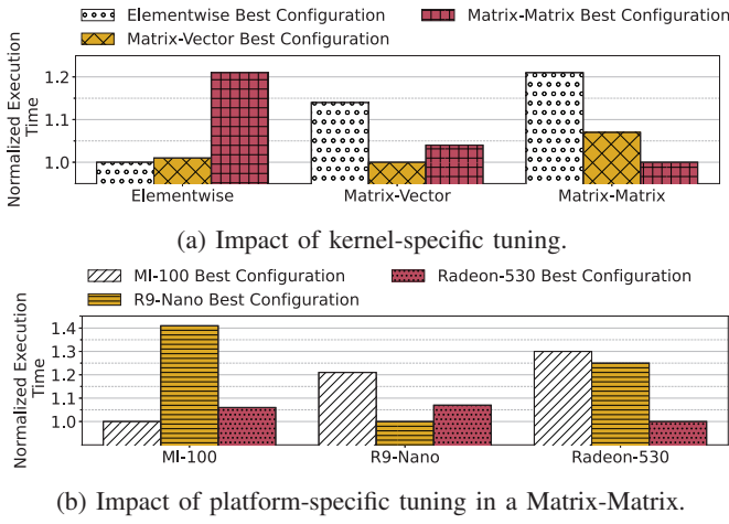
Fig. 1: Lack of portability of ATT tuning effort.
