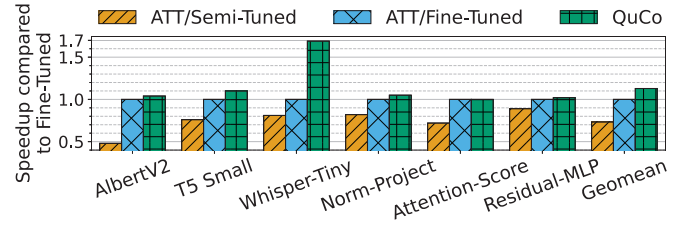
Fig. 8: Speedup over the ATT/Fine-Tuned baseline for several DNN models and composite kernel workloads
