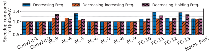
Fig. 12: QuCo-HW VS QuCo-SW over three different scenarios with varying frequency, see Section V-F for details.
