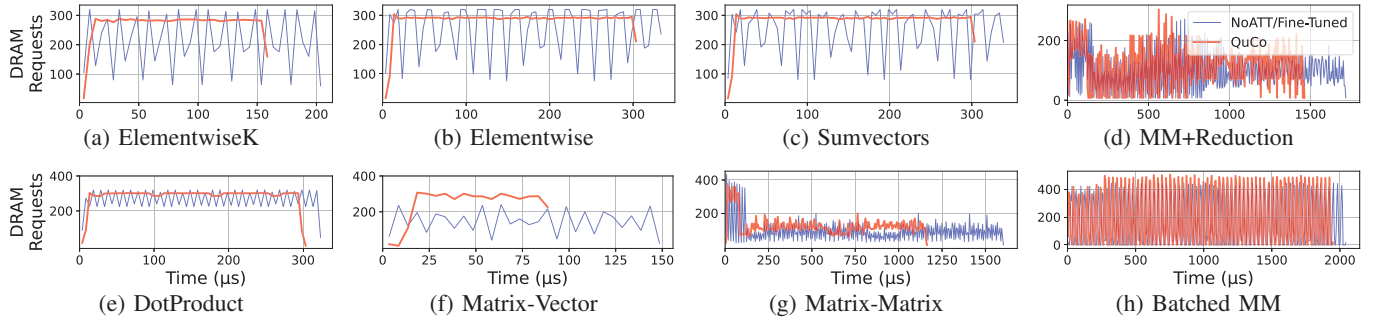
Fig. 5: DRAM activity over time for NoATT/Fine-Tuned and QuCo .
