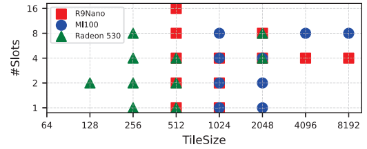
Fig. 11: Variance of QuCo parameters in the DNN models and composite kernels for the three GPUs.
