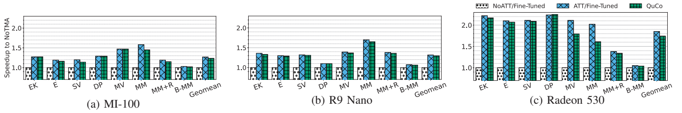
Fig. 10: Portability study: same post-compilation QuCo binary on GPUs with different compute and memory specs.
