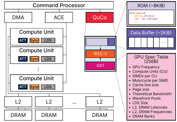
Fig. 3: Overview of the GPU architecture with the QuCo unit.
