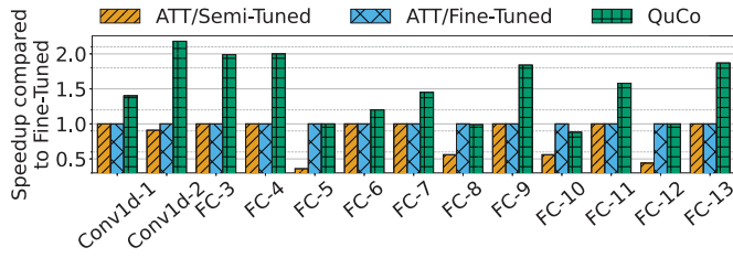
Fig. 9: Layer-wise speedup in the Whisper-Tiny model (singular layers) compared to the ATT/Fine-Tuned baseline
