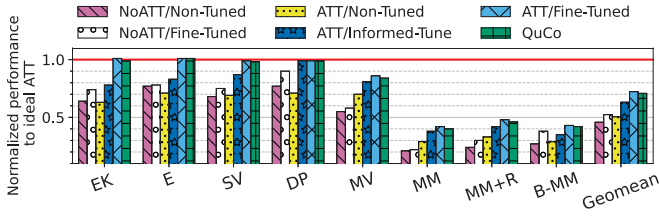
Fig. 6: Kernel execution normalized to the ideal scenario.
